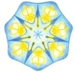
25-01 Merkur Saturn
