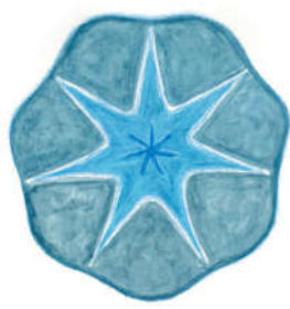
1-01 Saturn
