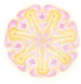
16-01 Mond Jupiter
