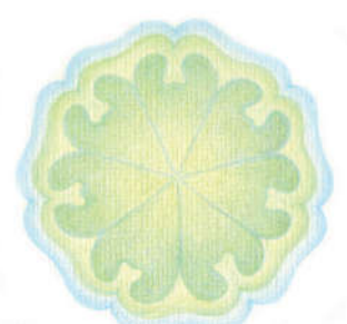
2-06 Venus
