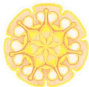
23-01 Merkur Jupiter
