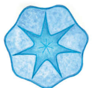
1-03 Saturn
