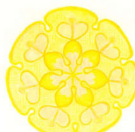
4-03 Merkur
